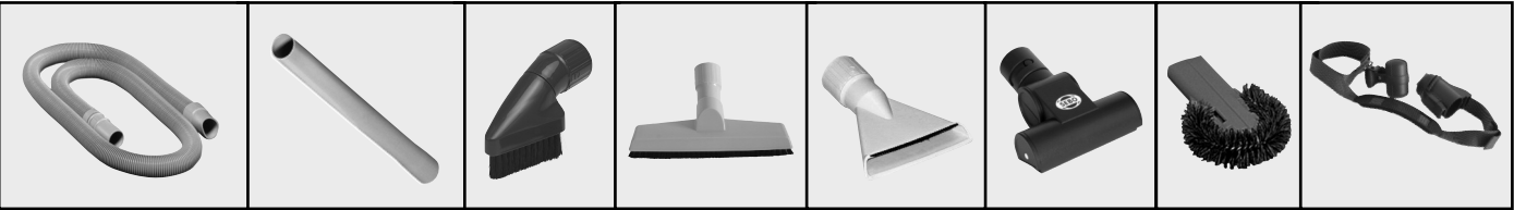
9-foot Extension Hose Part #1495AM 20-inch Extension Tube Part #1084HG Dusting Brush Part #1387DG Wall & Floor Brush Part #1325HG Flat Upholstery Nozzle Part #1090HG Hand-held Turbo Brush Part #6179DA Radiator Brush Part #1496DG Shoulder Strap Part #7158
